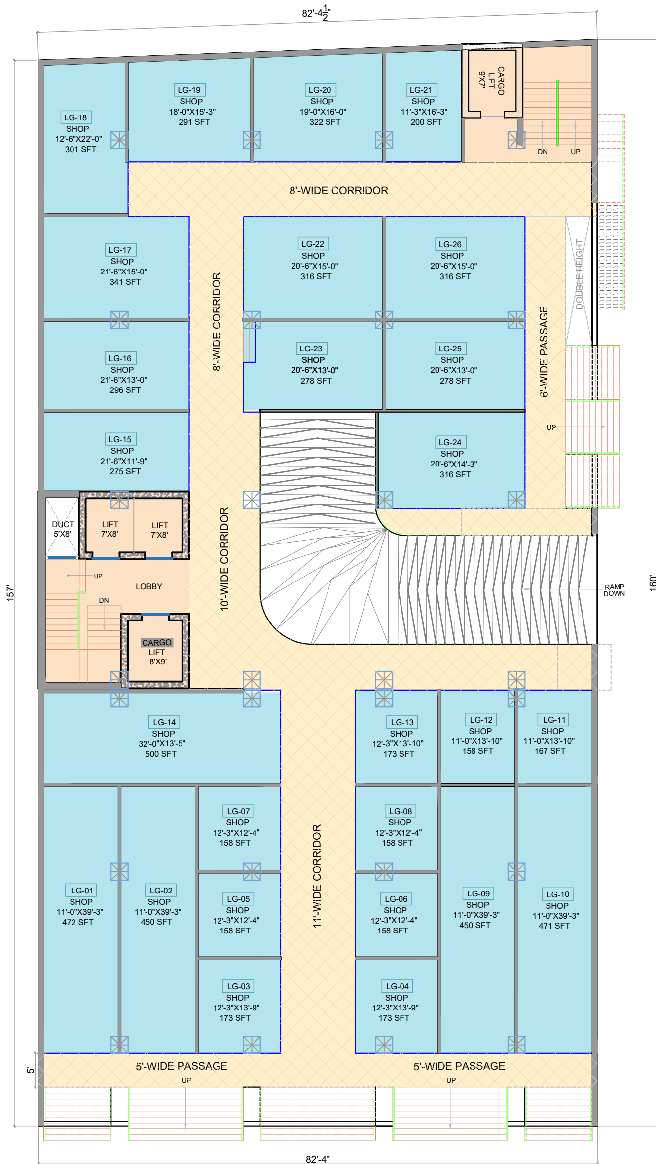
LOWER GROUND FLOOR PLAN SHOPS (26 NO'S)
