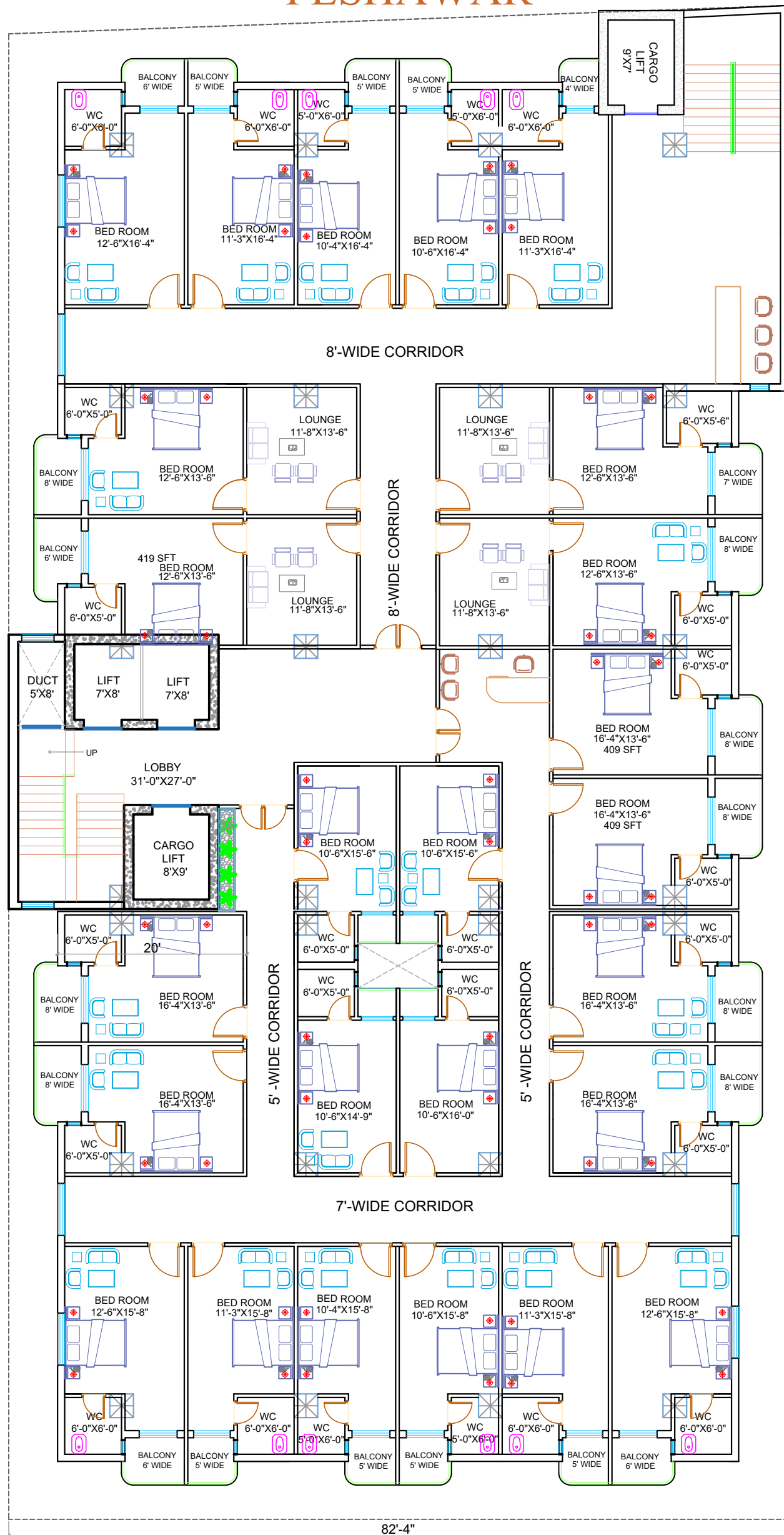
SIXTH FLOOR PLAN (FLATS AND HOTEL ROOMS)
