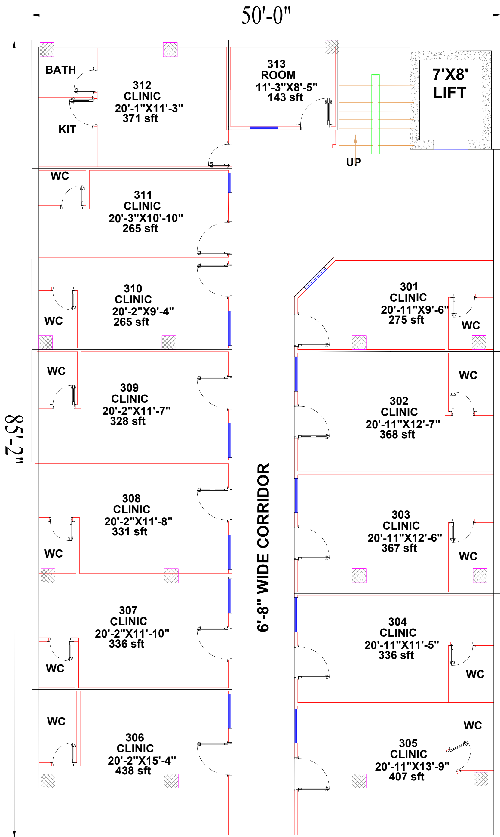
3rd FLOOR PLAN COVERED AREA= 4236 SFT
