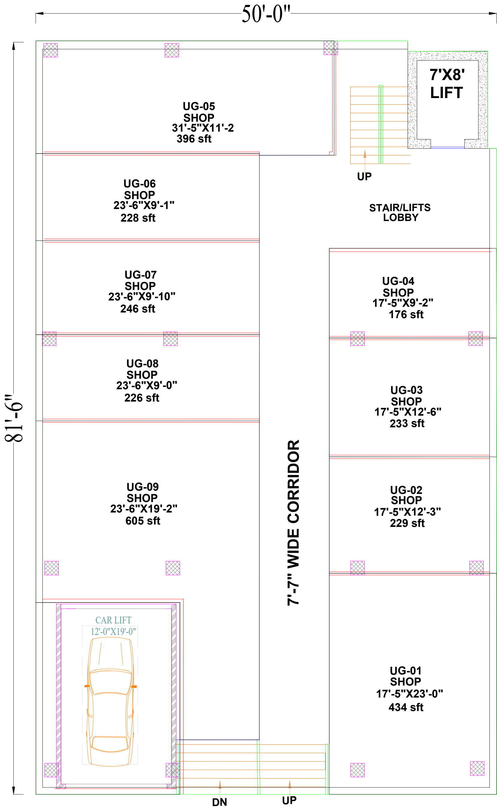
GROUND FLOOR PLAN COVERED AREA= 4060 SFT
