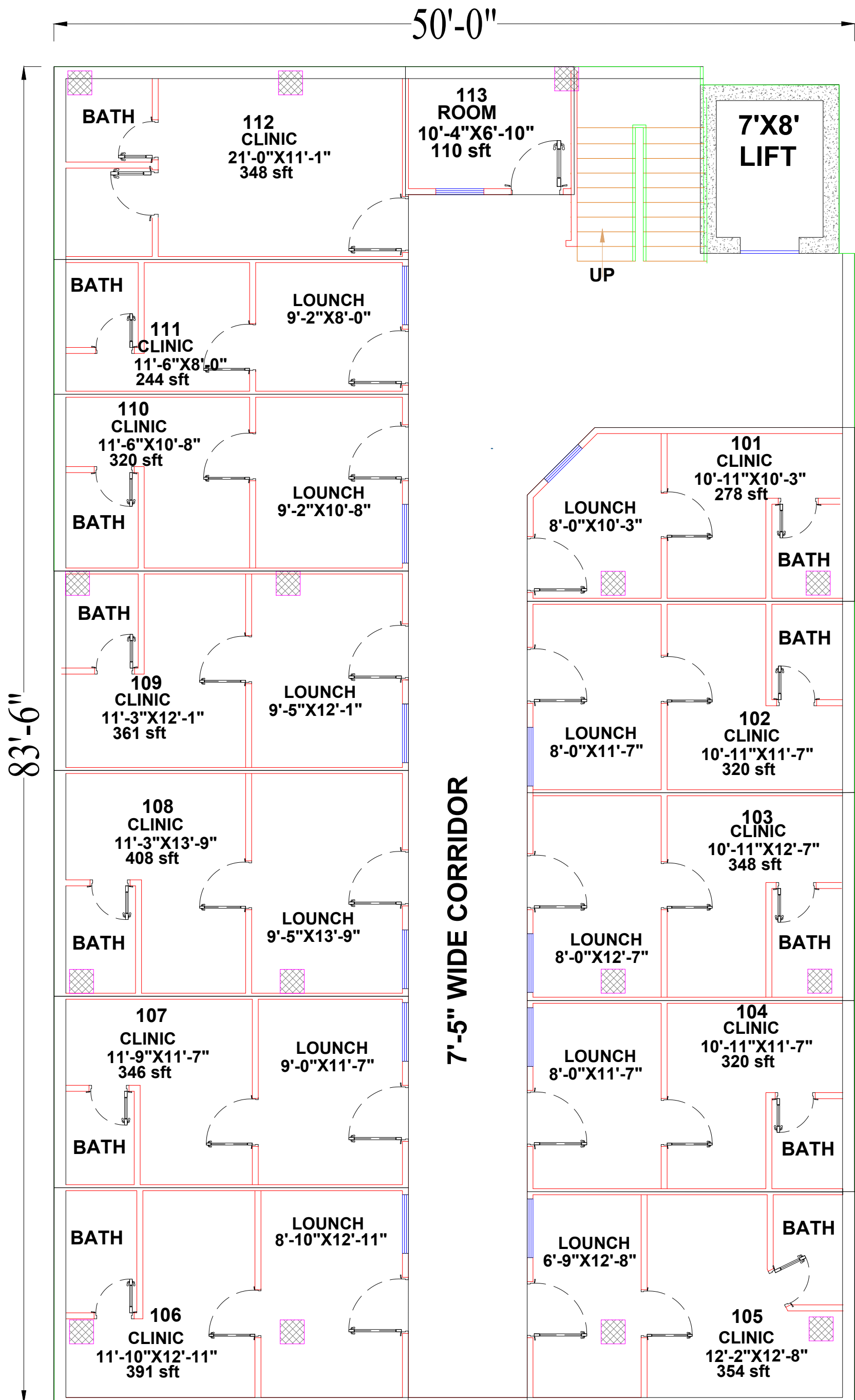
FIRST FLOOR PLAN COVERED AREA= 4152 SFT
