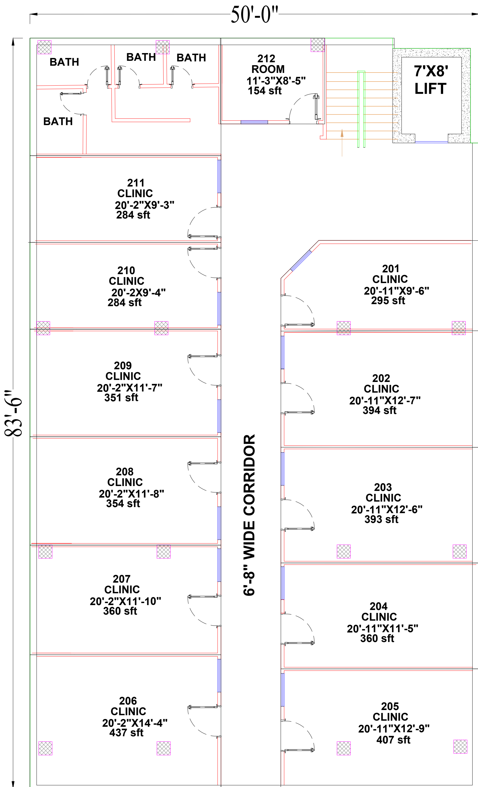
2ND FLOOR PLAN COVERED AREA= 4152 SFT
